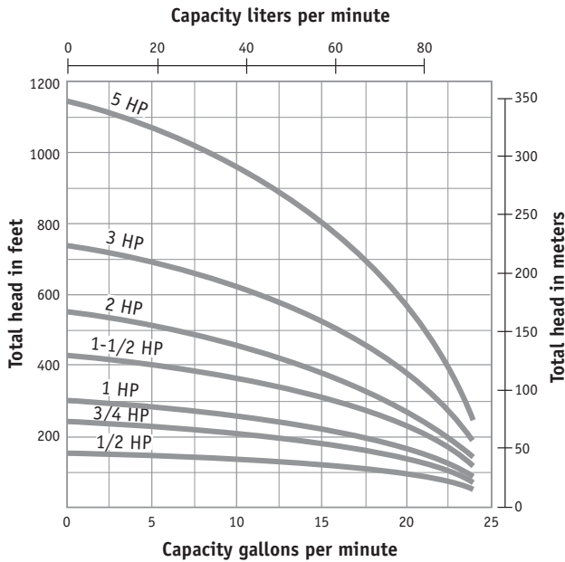
PUMP PERFORMANCE - 16 GPM
